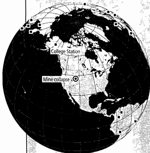
The collapse of a mine in southwestern Wyoming sent long-range seismic "body" waves around the world. (Body waves pass through the solid interior of Earth.) The waves were picked up by seismic stations at least 2,000 miles away (squares).
